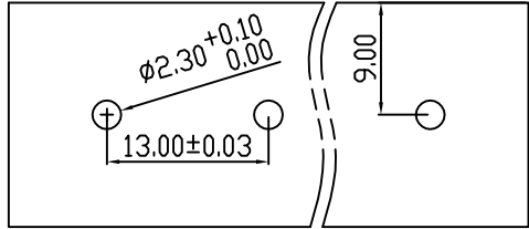
PCB LAYOUT
