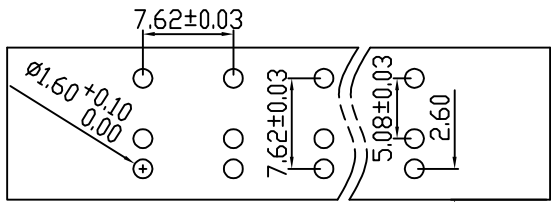
PCB LAYOUT
