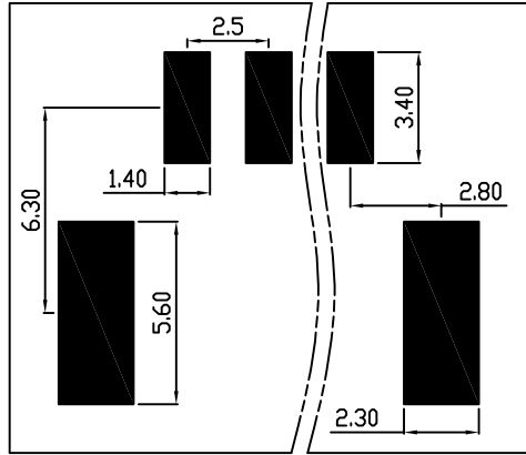
PCB Layout
