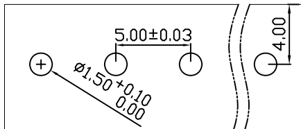
PCB LAYOUT
