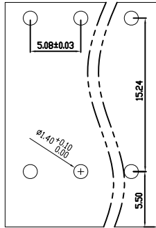
PCB LAYOUT
