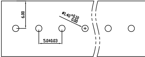
PCB LAYOUT
